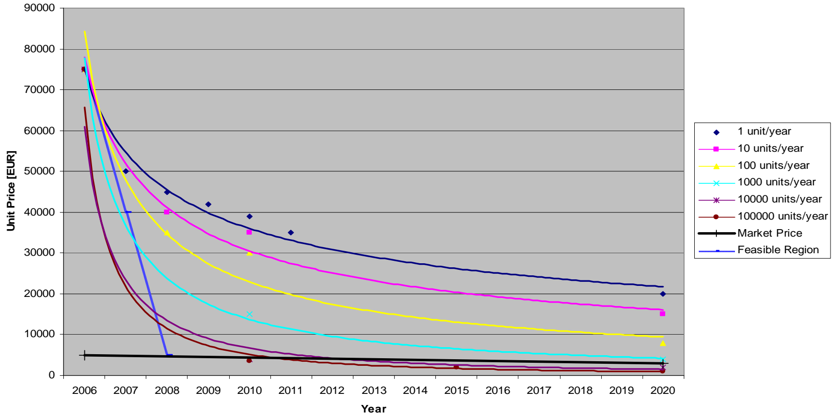
Learning Curve, 1 kW el, Pure Hydrogen, 40.000 Hours Lifetime
